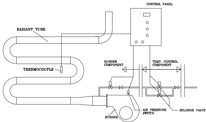
RADIANT TUBE BURNER
