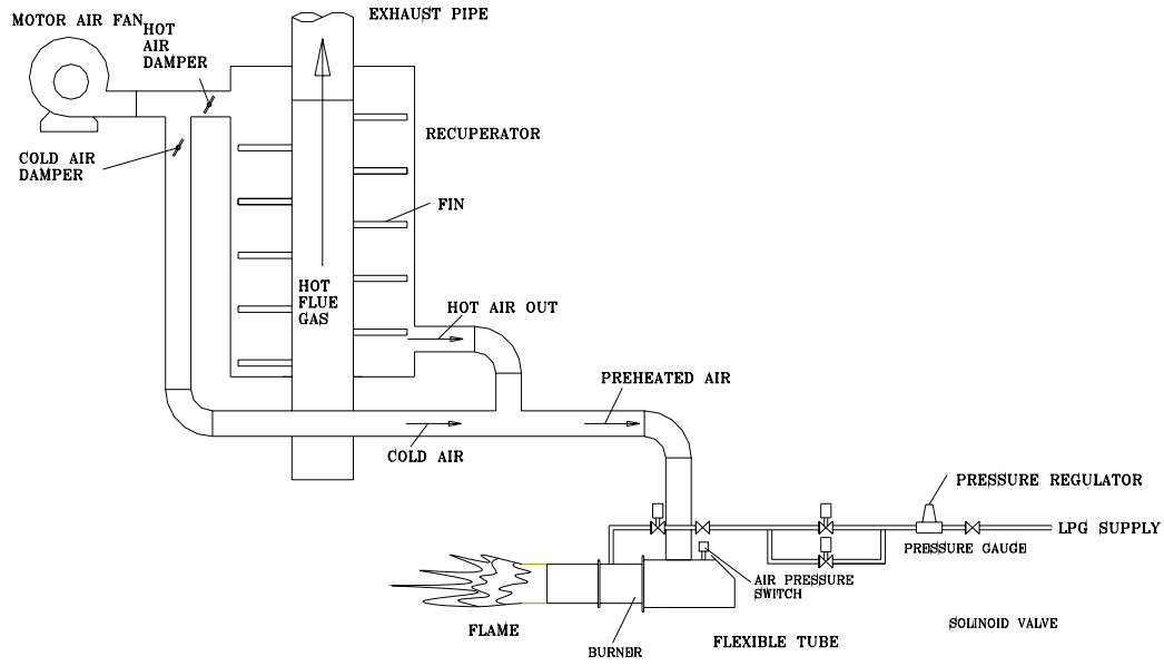
RECUPERATIVE BURNER
