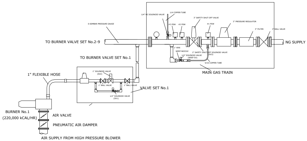
GAS TRAIN FOR 1,980,000 kCAL/HR NG (233 NM.3/HR)
