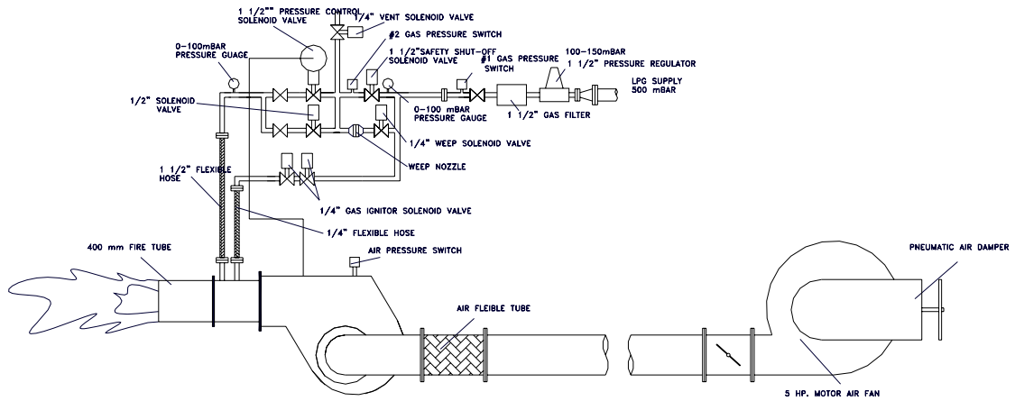
5 M BTU GAS BURNER
