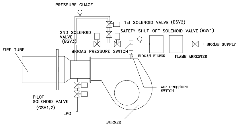
BKE BIOGAS BURNER
